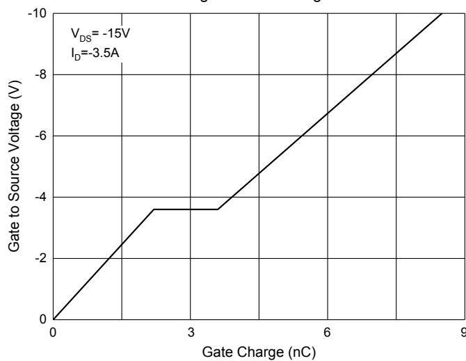
Fig. 5 - Gate Charge
