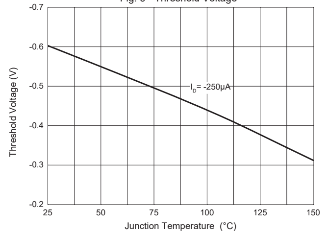
Fig. 6 - Threshold Voltage
