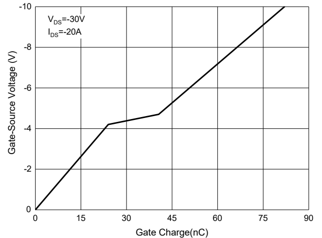
Fig. 6 - Gate Charge
